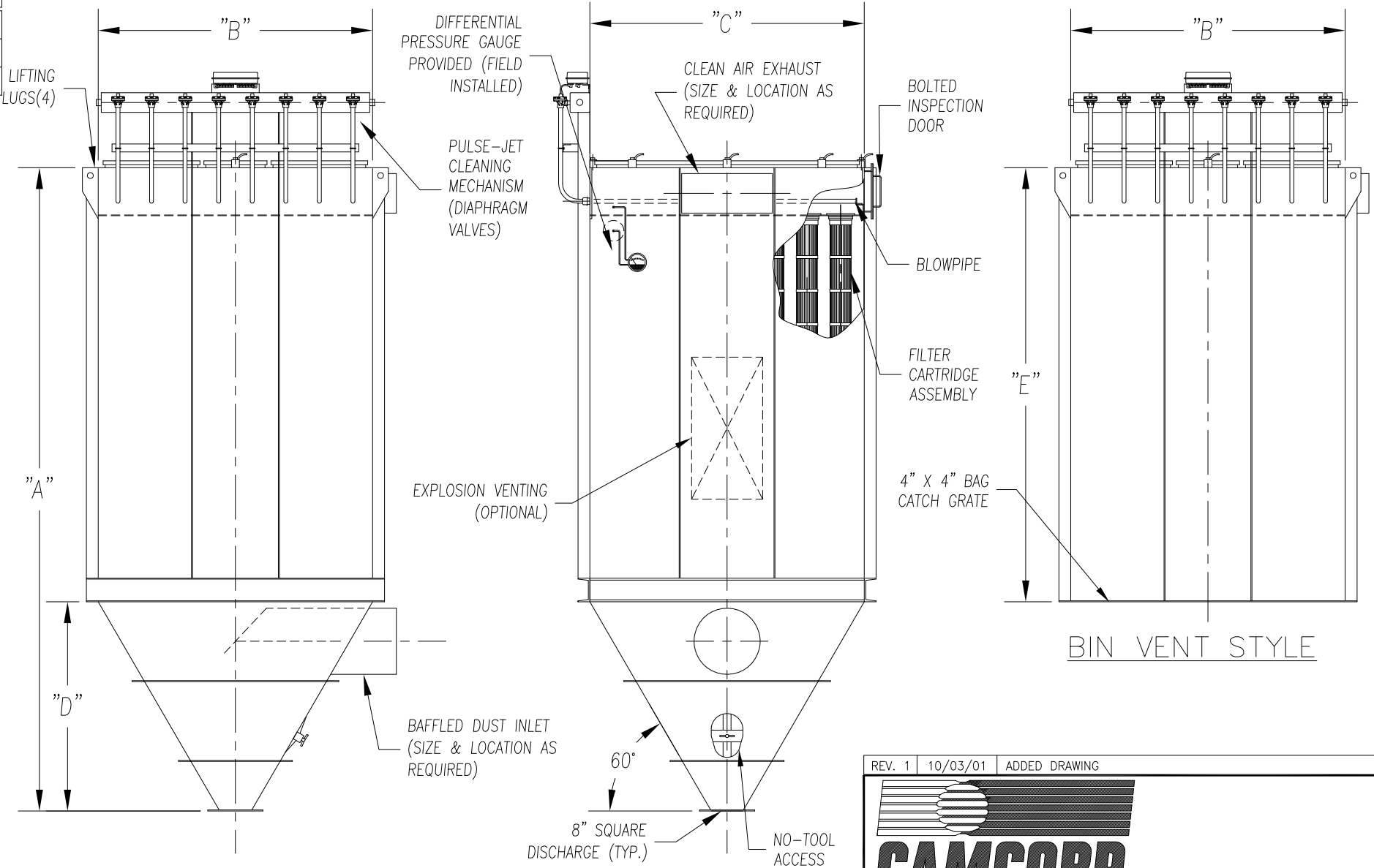
TOP REMOVAL CARTRIDGE DUST COLLECTOR ( 196 TO 256 CARTRIDGES )
